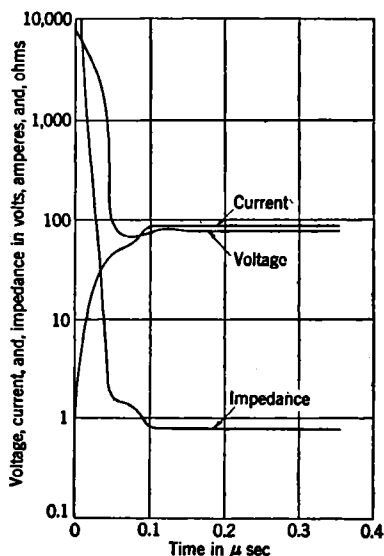
FIG. 8-43.—Tube drop, current, and impedance as a function of time for a 4C35 hydrogen thyatron ( V_N = 8 kv, I_p = 90 amp, \tau = 1.1 μsec).
